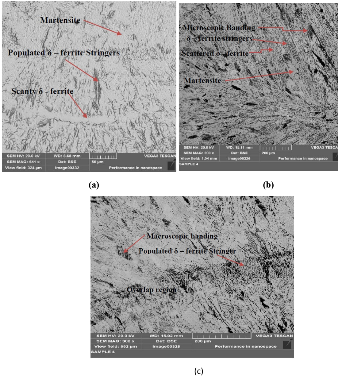
Figure 4. The (a)Microstructure of sample at low laser power 1000 KW (b) Microstructure of sample at high laser power 2200 KW. (c) Micrograph of Overlap region at high laser power 2200 KW.
