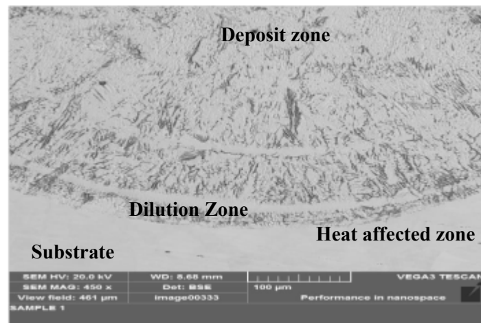
Figure3. Micrograph of Sample at a laser power of 1.0 kW
