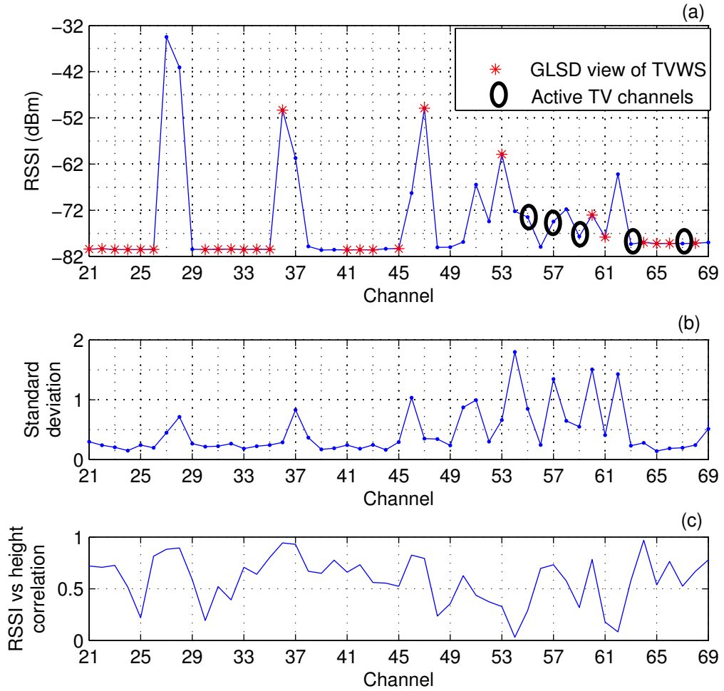
Fig. 2. Overview of the spectrum scan.
