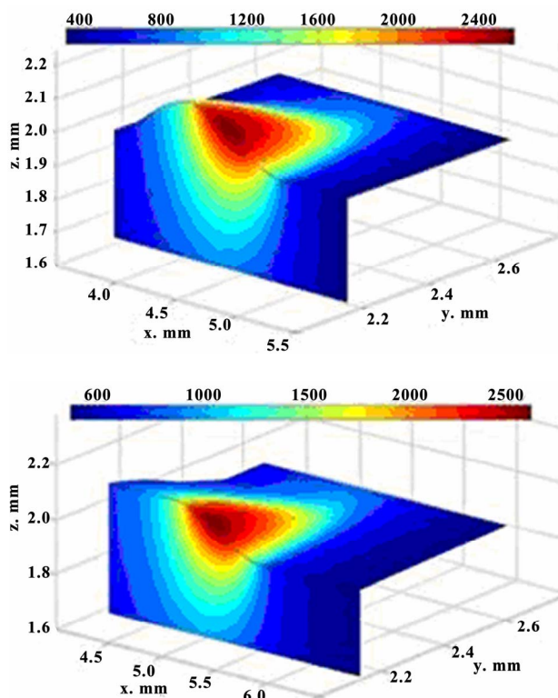
Figure 2. 3D dynamics of temperature fields; t = 62 ms (up) and t = 122 ms (down).
