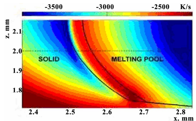
Figure 4. Spatial distribution of cooling rate in the crystallization zone P = 0.75 kW, t = 200 ms, V = 12 mm/s, m = 1 g/min.
