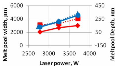
Figure 10. Experimental (dotted line) and numerical (solid line) values of melt pool width (red) and depth (blue) as a function of laser power. Feed rate m = 8.9 \text{ g/min} , scanning velocity V = 40 \text{ mm/min} .
