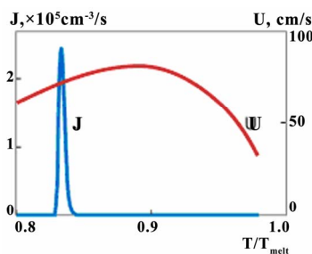
Figure 6. The temperature dependences of nucleation ( J ) and growth rates ( v ); t = 156 \text{ ms} .
