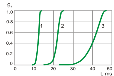
Figure 8. The time dependences of volume fraction of solid phase for different cooling rates. (1) 4500 K/s; (2) 2400 K/s, and (3) 1200 K/s.
