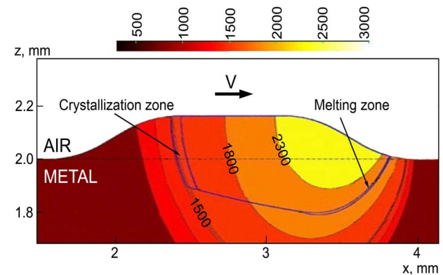
Figure 3. The x - z cross-section of temperature field, t = 130 m/s.
