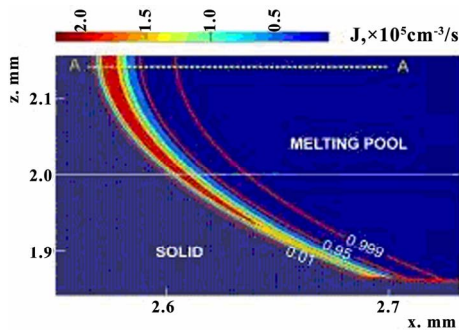
Figure 5. The x-z cross-section distribution of nucleation rate, t = 156 \text{ ms} .
