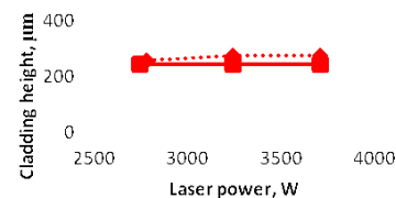
Figure 9. Clad height dependence on laser power. Dotted curve is experiment, solid line is numerical calculations. feed rate m = 8.9 \text{ g/min} , scanning velocity V = 40 \text{ mm/min} .
