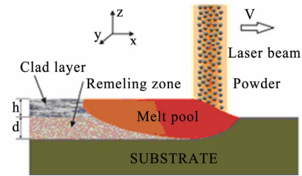
Figure 1. The scheme of laser cladding by powder injection.
