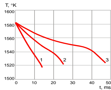
Figure 7 The temperature dynamics for different cooling rates. (1) 4500 K/s; (2) 2400 K/s; and (3) 1200 K/s.
