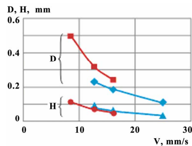
Figure 11. Melt pool depth ( D ) and clad height ( H ) dependence on scanning speed for different laser power ( \blacklozenge, \blacktriangle — P = 0.6 \text{ kW} ; \blacksquare, \bullet — P = 0.75 \text{ kW} ).
