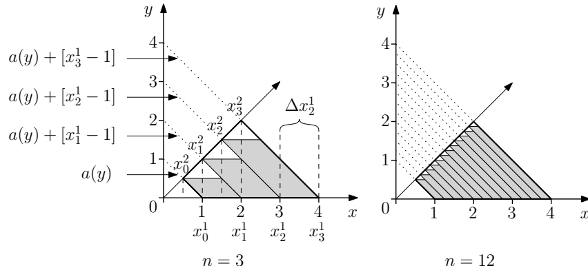
Figure 13: Partition points x_i^2 as used in the Cavalieri sum.
