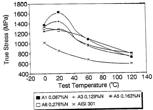
FIGURE 3. True stress at 0,3 strain as a function of temperature for alloys A1, A3, A5, A6, and type 301.
