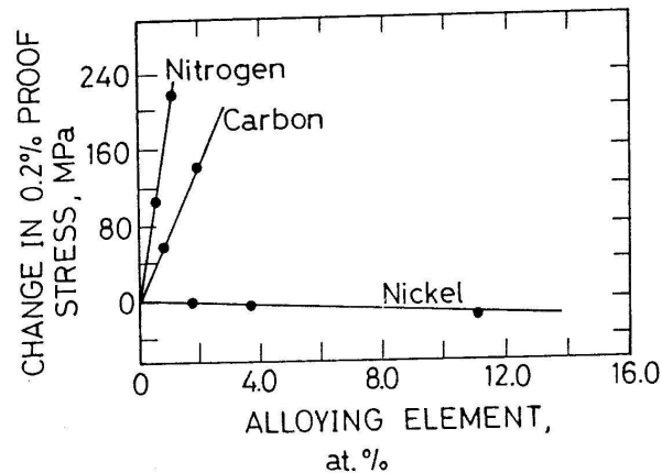
Figure 5.9 Yield strengthening ability of nitrogen compared to that of carbon and nickel (42) .
