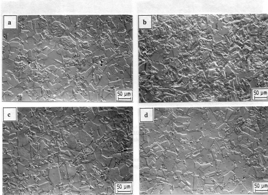
Figure 4.2 Microstructures of set 47, solution-treated at 1050°C for 30 minutes followed by oil quench. Electro-polished and electro-etched. Surface relief enhanced by Nomarski interference contrast.
