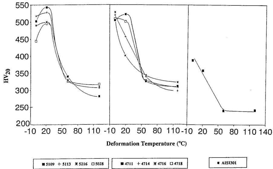
Figure 4.21 Bulk hardness of experimental alloys and type 301, at 0.3 true strain.
