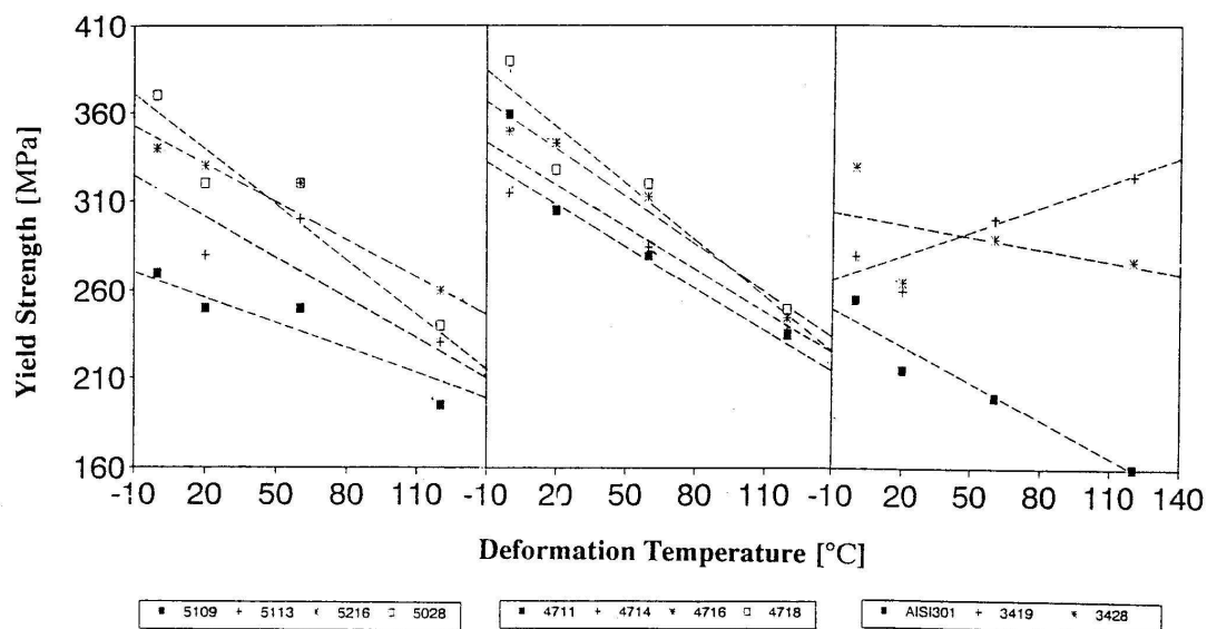
Figure 4.28 Yield strength of experimental alloys and the type 301 alloy, as a function of temperature.
