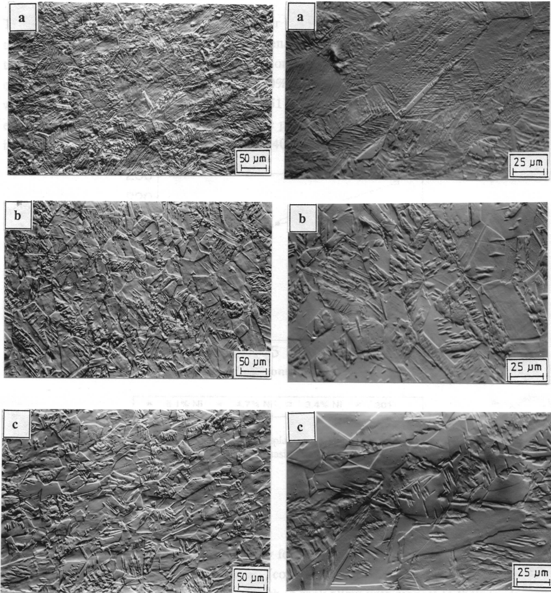
Figure 4.19 Type 301 deformed to 0.3 true strain at:
