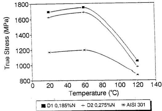
FIGURE 4. True stress at uniform strain ( \sigma_u ) as a function of temperature (set D alloys and type 301)
