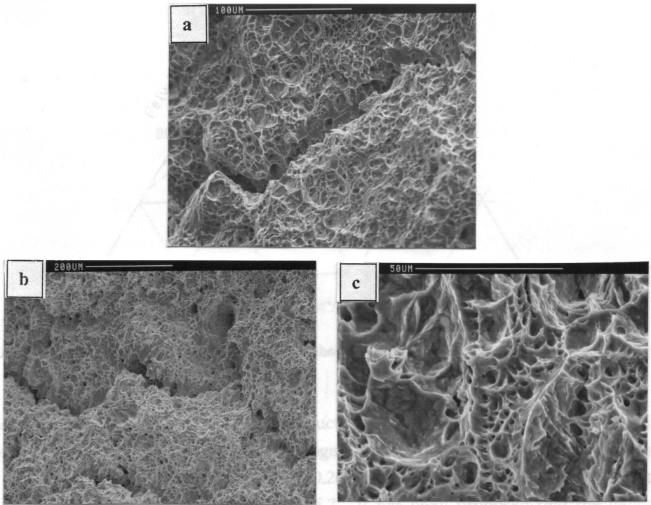
Figure 4.34 Impact fracture surfaces of tests at 20°C.
