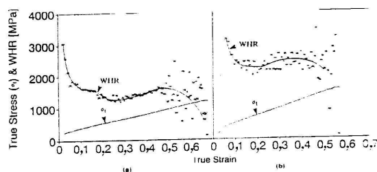
FIGURE 8. (a) Work-hardening rate (WHR) of type 301 as a function of true strain at 60 °C (b) Work-hardening rate (WHR) of alloy A5 as a function of true strain at 60 °C
