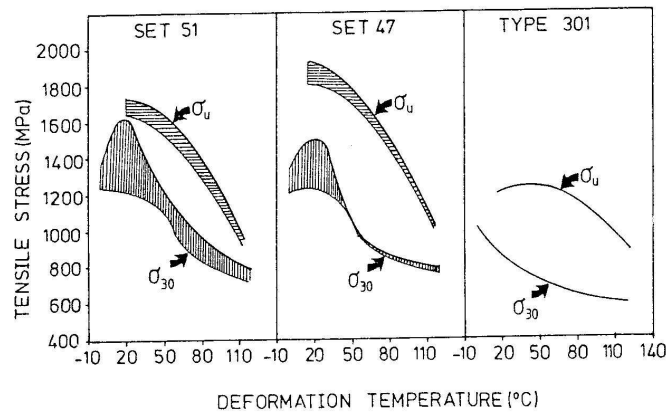
Figure 5.10 Tensile stress at 0.3 strain ( \sigma_{30} ) and at maximum uniform strain ( \sigma_u ) of sets 51 and 47, and the type 301 alloy, as a function of temperature.
