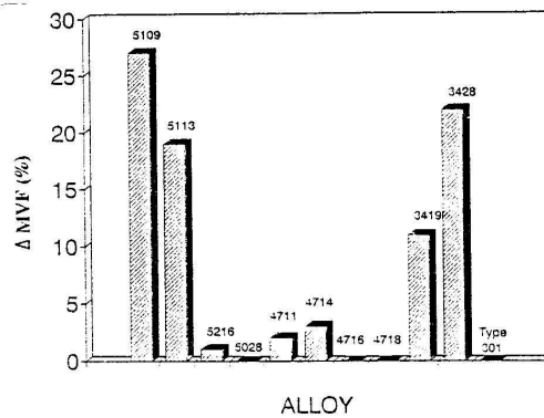
Figure 3.10 \Delta\text{MVf} of solution-treated, undeformed alloys determined using CuK \alpha and MoK \alpha radiation.
