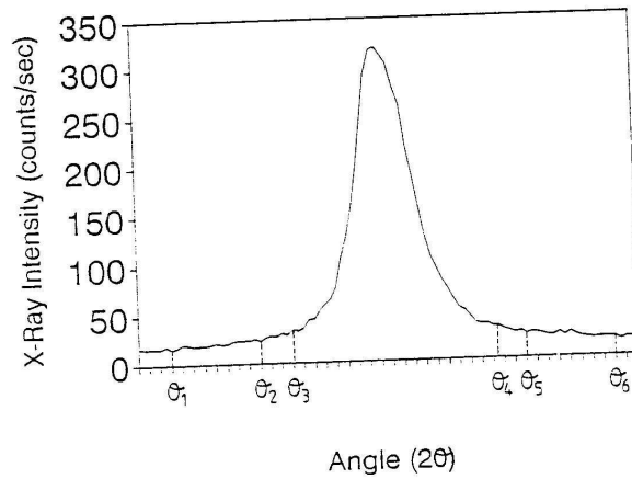
Figure 3.7 Determination of left and right peak angles ( \theta_3 and \theta_4 ), as well as angles for determining the left and right backgrounds ( \theta_1 , \theta_2 , \theta_5 and \theta_6 ).
