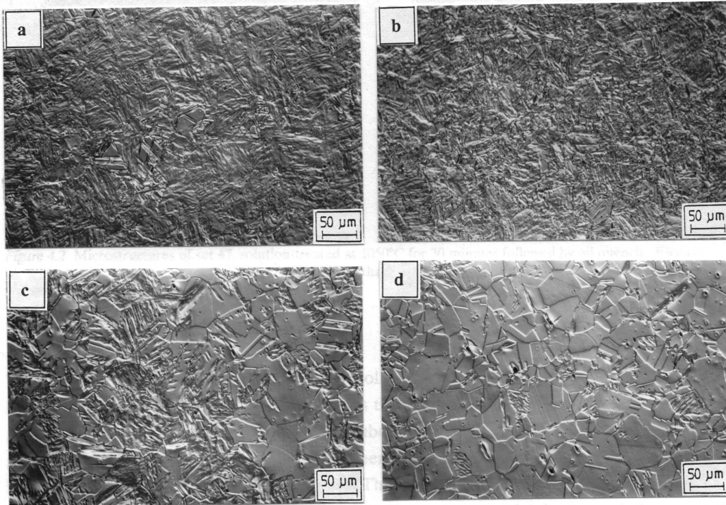
Figure 4.1 Microstructures of set 51, solution-treated at 1050°C for 30 minutes followed by oil quench. Electro-polished and electro-etched. Surface relief enhanced by Nomarski interference contrast.
