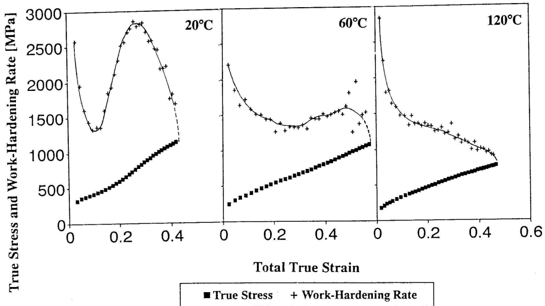
Figure 4.9 Work-hardening rate and true stress as a function of true strain : Type 301 deformed at 20, 60 and 120°C.
