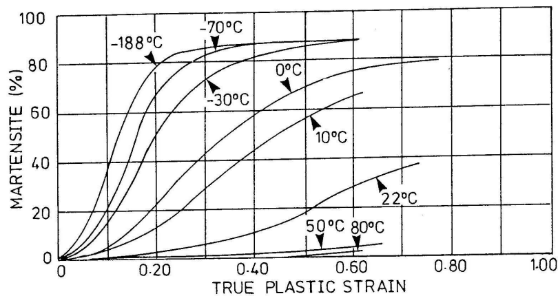
Figure 2.3 Formation of martensite by plastic tensile strain at various deformation temperatures (13) .
