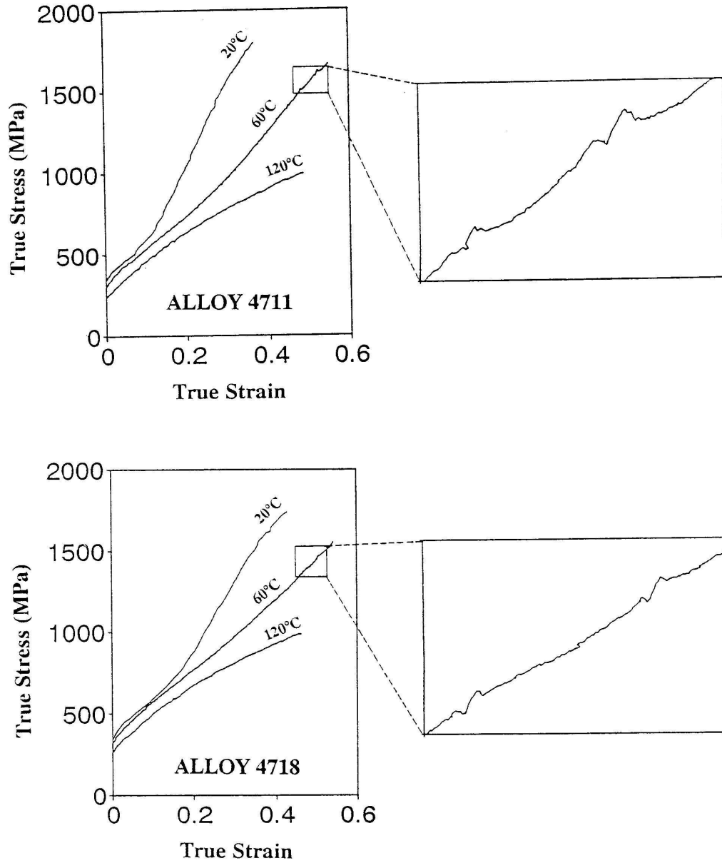
Figure 4.8(c) True stress-true strain curves of set 47 alloys at 20, 60 and 120°C. Pronounced serrations at 60°C occur in both alloys, but are smaller in alloy 4718.
