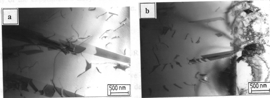
Figure 4.6 Alloy 4718 (a) Bright field image showing partial dislocations separated by stacking faults. No nitrides are evident. (b) Bright field image showing martensitic region adjacent to austenitic region.
