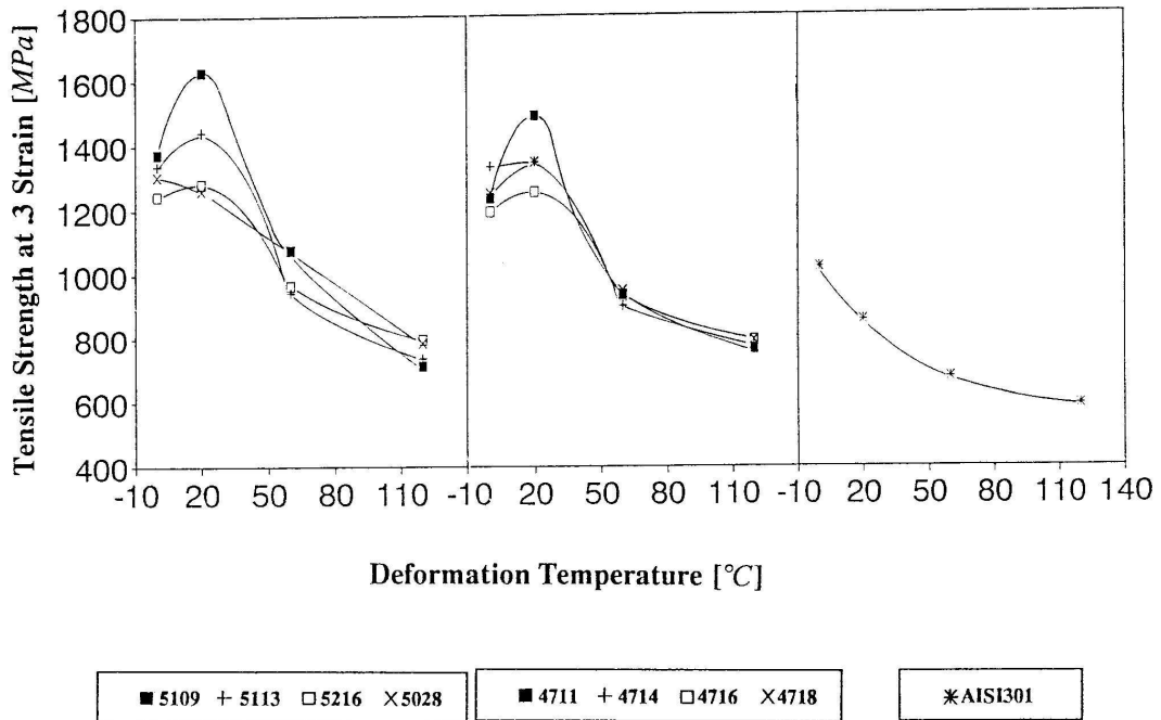
Figure 4.29 True stress at 0.3 true strain of experimental alloys and the type 301 alloy as a function of temperature.
