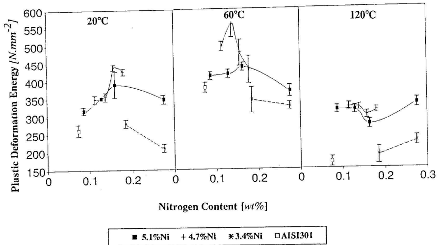
Figure 4.23 Plastic deformation energy of experimental alloys and the type 301 alloy absorbed between yield strain and e_u , as a function of nitrogen content.
