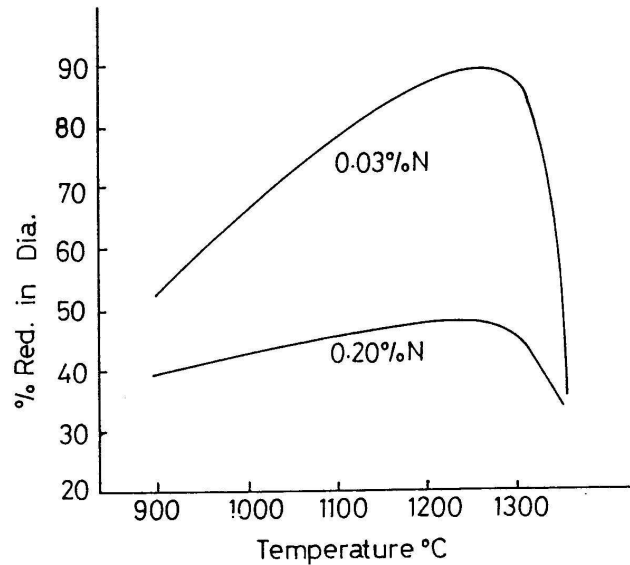
Figure 5.2 The effect of nitrogen content on the hot workability of austenitic stainless steels containing no \delta -ferrite (42) .
