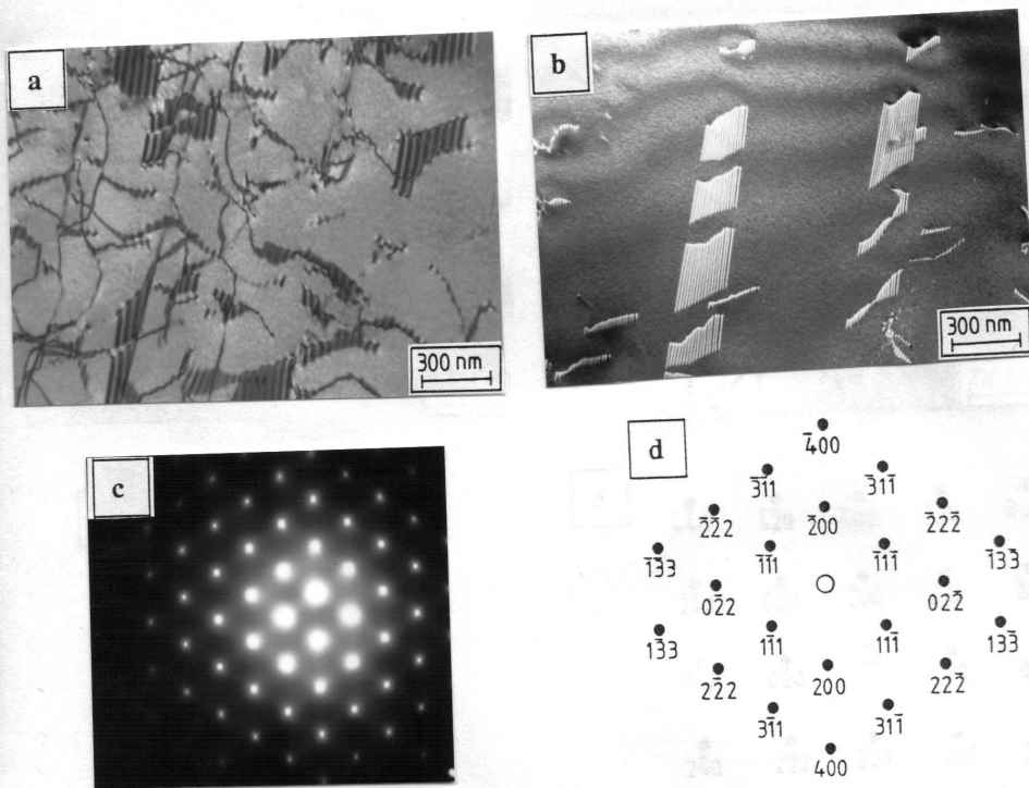
Figure 4.5 Alloy 5028 (a) Bright field image showing partial dislocations separated by stacking faults. (b) Dark field image showing co-planar arrays of partial dislocations separated by stacking faults. (c) Diffraction pattern along [011] zone axis. Note the absence of diffraction spots corresponding to nitride precipitates. (d) Diffraction index map of (c).
