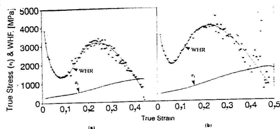
FIGURE 7. (a) Work-hardening rate (WHR) of type 301 as a function of true strain at 20 °C (b) Work-hardening rate (WHR) of alloy A5 as a function of true strain at 20 °C
