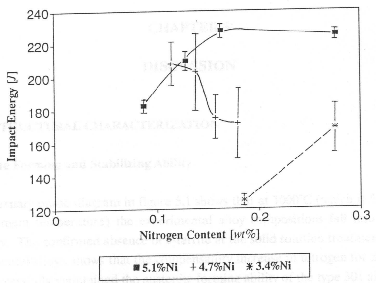
Figure 4.33 Impact energy absorbed by experimental alloys at room temperature.
