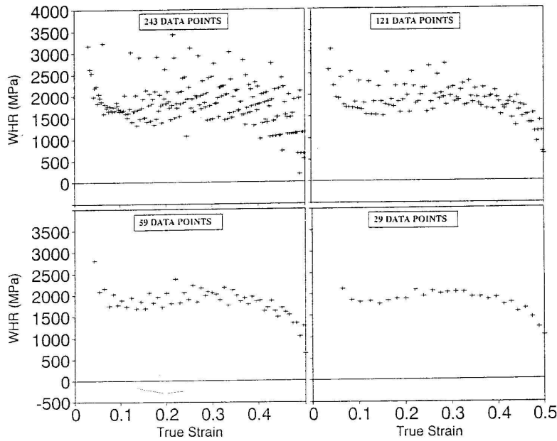
Figure 3.4 Systematic elimination of alternate data points to produce a smooth work-hardening rate curve.
