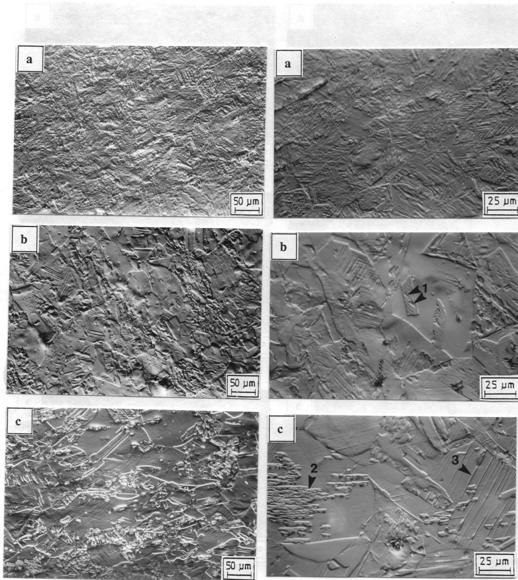
Figure 4.18 Alloy 4718 deformed to 0.3 true strain at:
