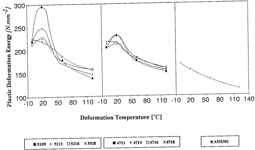
Figure 4.22 Plastic deformation energy of experimental alloys and the type 301 alloy absorbed between the yield strain and 0.3 true strain, as a function of deformation temperature.
