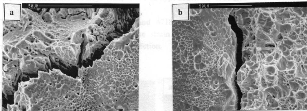
Figure 4.15 Fracture surface of tensile test at 20°C:
