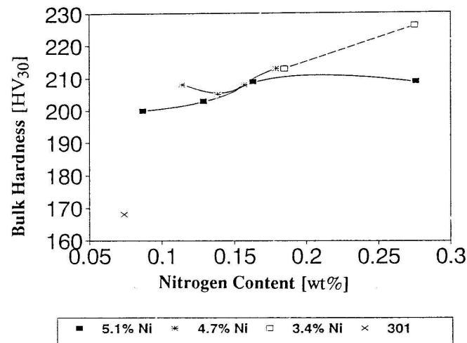
Figure 4.20 Bulk hardness of sets 51, 47 and 34 displaying the effects of decreasing martensite content and increasing solid solution hardening, with increasing nitrogen content.
