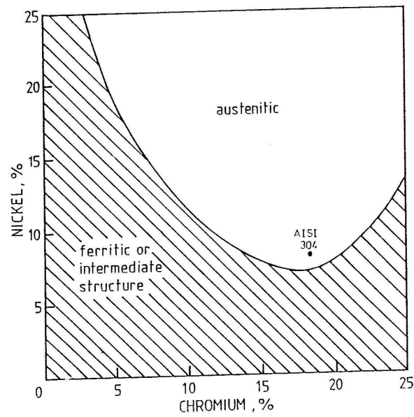
Figure 2.1 Effect of nickel and chromium on the constitution of 0.1% C steels at 900°C. At 18% Cr the amount of nickel required for an austenitic microstructure is a minimum and is approximately 8% (10) .
