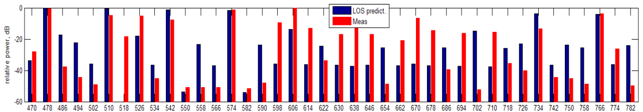
Figure 5: Max signal strength per TV channel - bar plot comparing the measured and simulated data side by side
