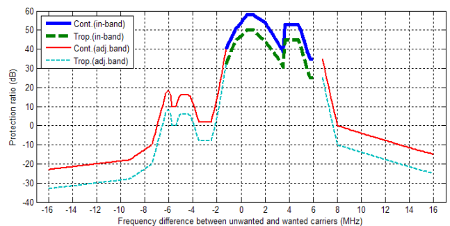
Figure 2: Protection ratio for PAL/I channels [11].
