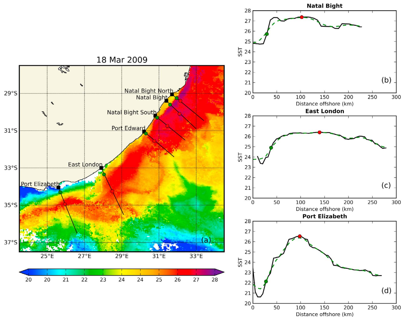
Figure 1. Example of output from the Agulhas front detection algorithm applied on a 3 day average map of SST (in ^{\circ}\text{C} ) centered around 18 March 2009. (a) A color contour map of SST over the region of study. The position of the Agulhas Current was tracked along six transects plotted as thin black lines and referenced to as Natal Bight North, Natal Bight, Natal Bight South, Port Edward, East London and Port Elizabeth. The position of the Agulhas Current core detected using the algorithm is plotted with a red dot while a green dot shows the position of the detected Agulhas Current inshore front. SST as well as the identified Agulhas Current core and inshore front positions are plotted for three selected transects at the (b) Natal Bight, (c) East London and (d) Port Elizabeth. The solid black lines in Figures 1b, 1c and 1d correspond to the SST along the transect, while the dotted green line shows the smoothed SST profiles used for the estimation of the Agulhas Current core's position.
