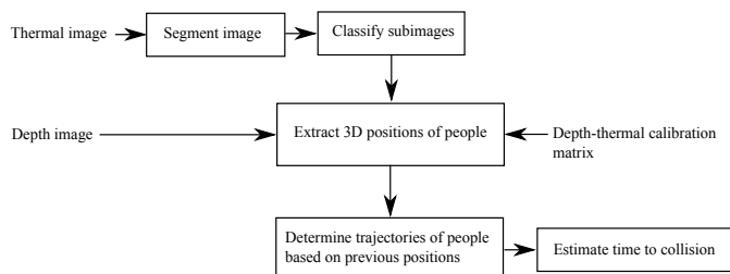
Fig. 1. A block diagram showing the subsystems making up the pedestrian detection system.
