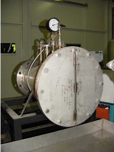
Fig. 1: Setup of pressurised vessel
