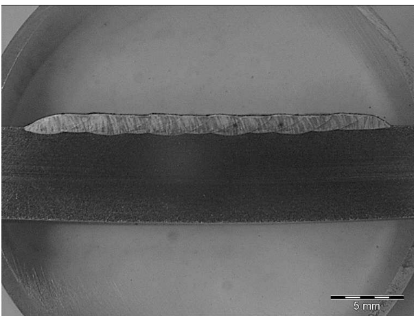
Fig. 8: Cross section of crack seal, 6.0 mm thickness
