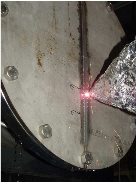
Fig. 5: Crack sealing of 6.0mm plate @ 2 bar pressure
