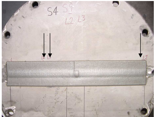
Fig. 6: Crack sealing and overlay of 6.0mm plate
