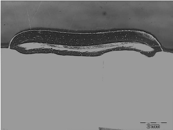
Fig. 7: Cross section of crack seal, 6.0 mm thickness
