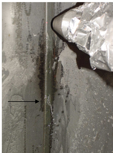
Fig. 3: Crack sealing without peening prior to cladding
