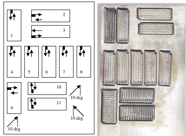
Fig. 2: Overlay positional welding
