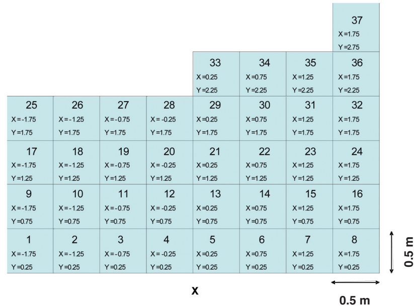
Figure 12—Plan view of the grid layout across the pillar for Boussinesq evaluation. The origin is the centre of the bottom (down-dip) edge. The bold “X” position represents the approximate position of the first stress measurement
