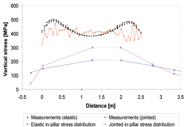
Figure 15—Distribution of stresses in the pillar centre and at in situ measurement positions for both the elastic and jointed models
