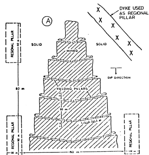
Figure 1—Plan view of a typical breast stope
