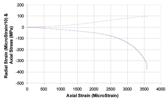
Figure 8—Stress-strain curve of the anorthosite rock above the instrumented pillar, provided by a laboratory UCS test
