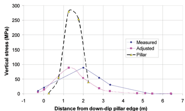
Figure 17—Stress profiles across the centre of the pillar, comparing the measured to the calculated
