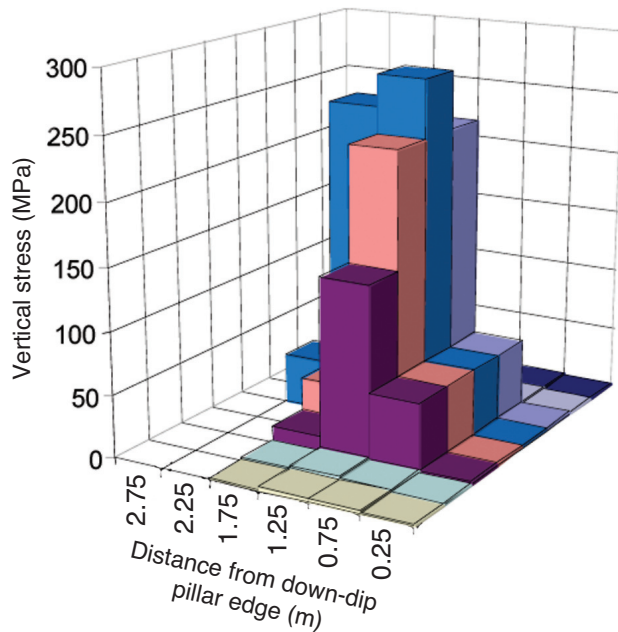
Figure 18—Stress profile across the pillar (provided by the Boussinesq inverse matrix)
