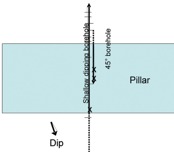
Figure 6—Plan view showing the instrumentation positions above the pillar (not drawn to scale). X=triaxial cells, —=biaxial cells
