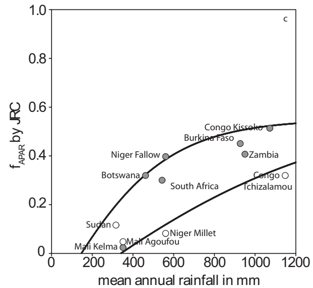
Fig. 8c. The relationship of satellite-derived f_{APAR} to mean annual rainfall for the analysed sites. The tree dominated ecosystem ( n=6 , grey, Mali-Kelma excluded) lie along the capacity curve, levelling of at 800 mm of rainfall ( y=0.75 \cdot \tanh(y(x \cdot 0.0014/0.75) - 0.2) ) and the grasslands ( n=4 , white) are explained by the curve below ( y=0.8 \cdot \tanh(y(x \cdot 0.0006/0.8) - 0.2) ).
