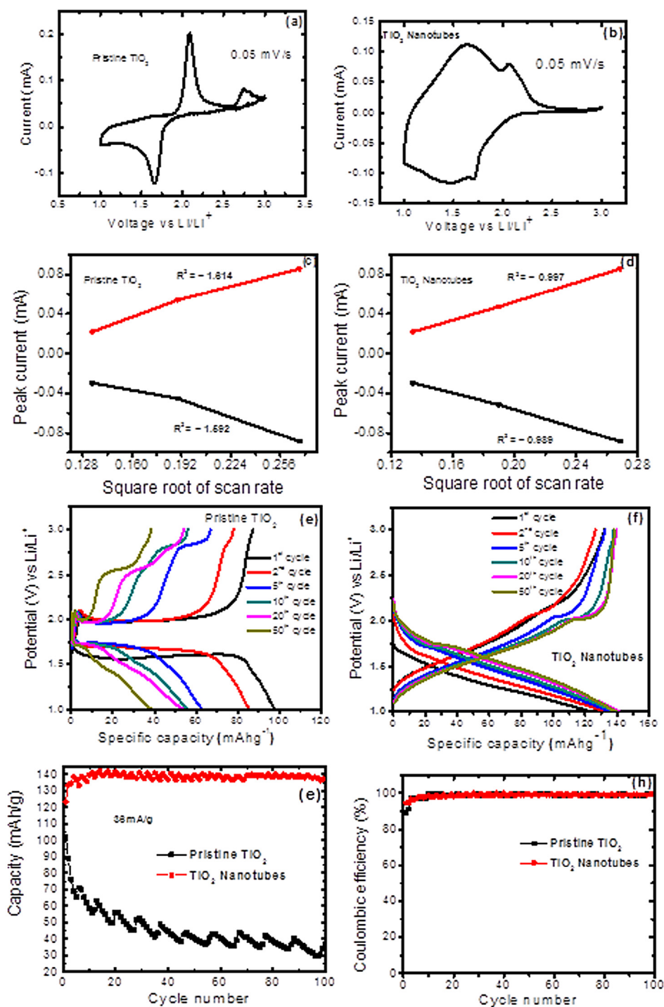
Fig. 5. (a–b) Cyclic Voltammetry curves of pristine TiO 2 and prepared TiO 2 nanotubes, (c–d) plot of anodic and cathodic peak current against square root of the scan rate for pristine TiO 2 and TiO 2 nanotubes, (e–f) CD curves of pristine TiO 2 and prepared TiO 2 nanotubes, (g) Performance of prepared TiO 2 nanotubes and pristine TiO 2 at 36 mA g -1 in the 1–3 V potential window and (h) Coulombic efficiency against cycle number of prepared TiO 2 nanotubes and pristine TiO 2 .
