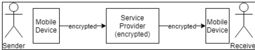
Figure 1. End-to-end Encryption
