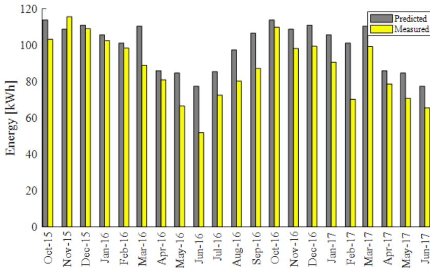
Figure 7: Comparison of monthly predicted and measured values of the electricity production
